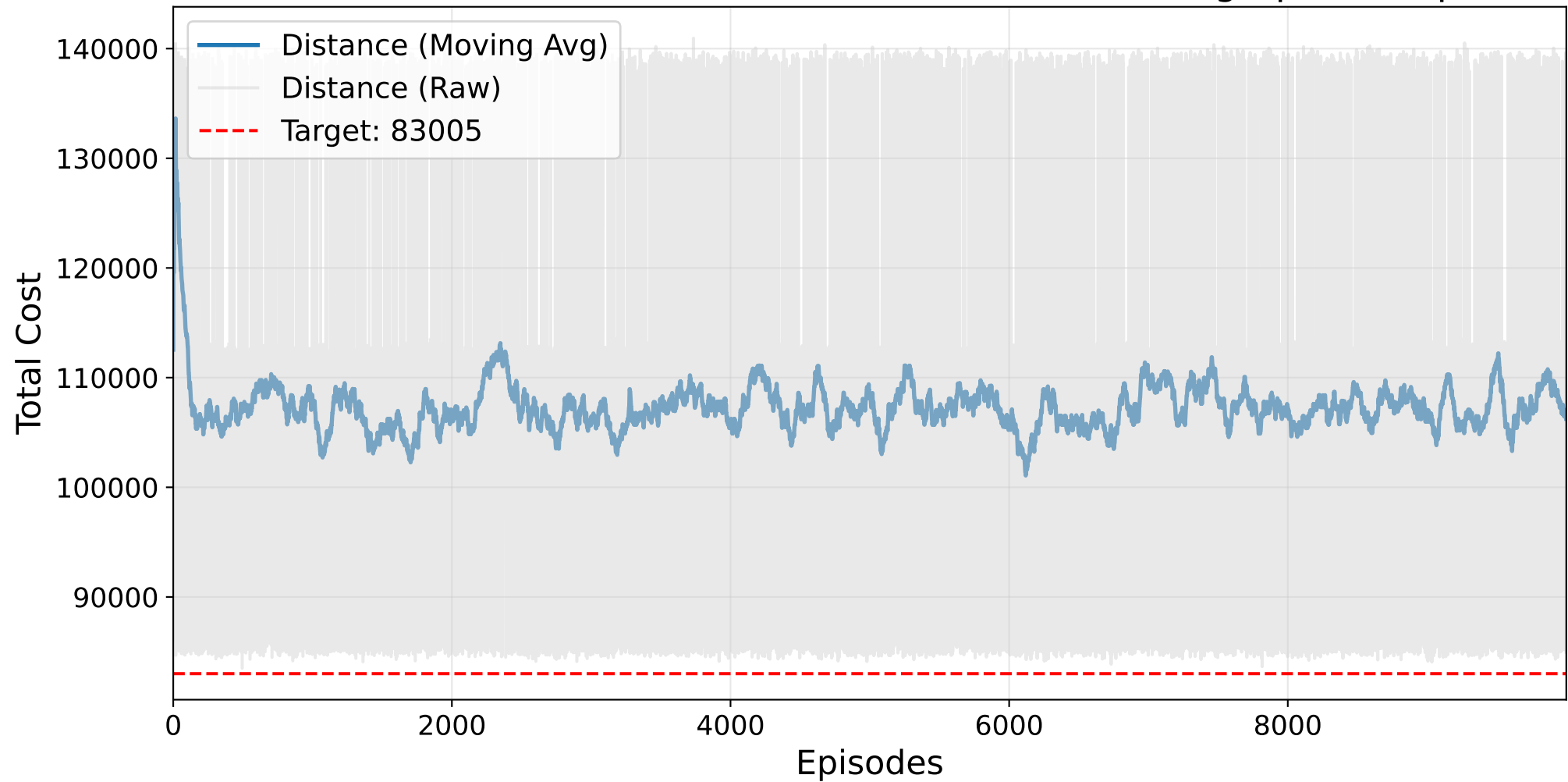
Final HYPERBAND TPE Masked AutoRL-SOP Training - p43.4.sop
